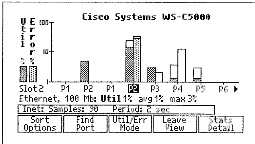
Figure 9-5. MultiPort Statistics
